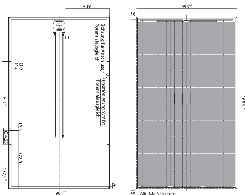
SCHOTT POLY™ 217/220/225/230/235
